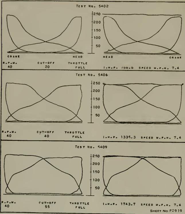
INDICATOR DIAGRAM, CLASS IIS TYPE LOCOMOTIVE.
